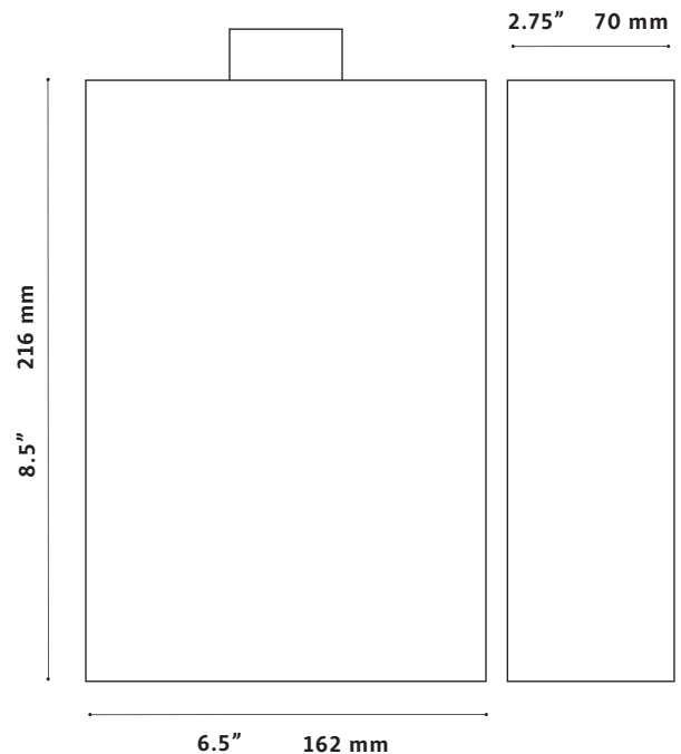
HANG TAB 1.875" x 1" 47.625 x 25.4 mm
